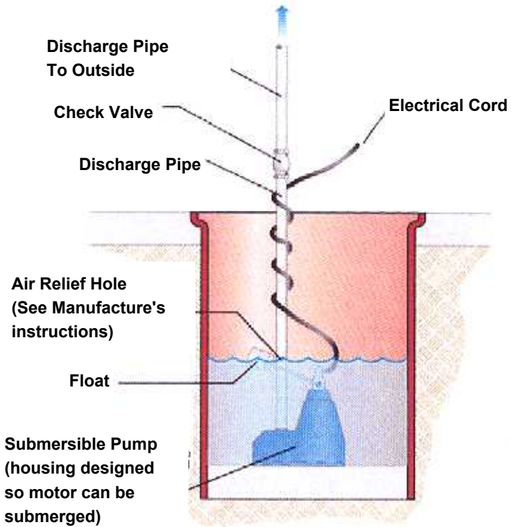
Submersible Pump
