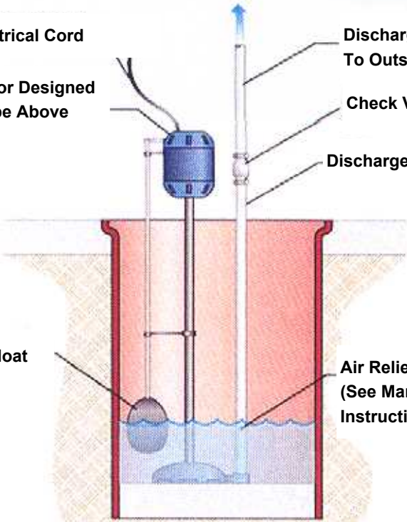
Pedestal Pump
